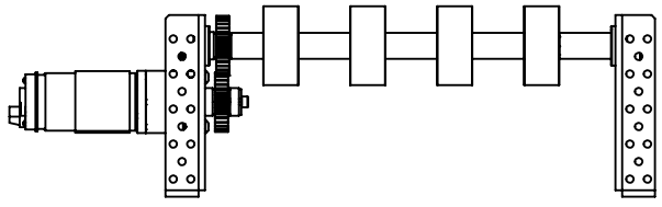
ASSEMBLED VIEW
