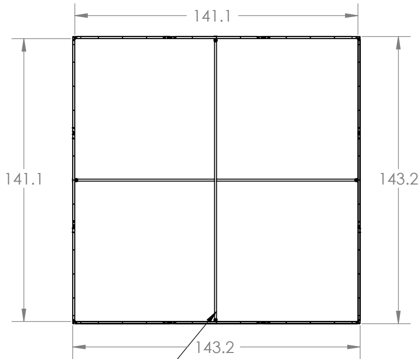
FIELD STRAPS (2)
