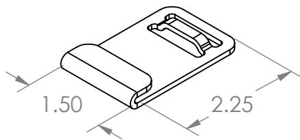
FIELD STRAP CLIP (4)
