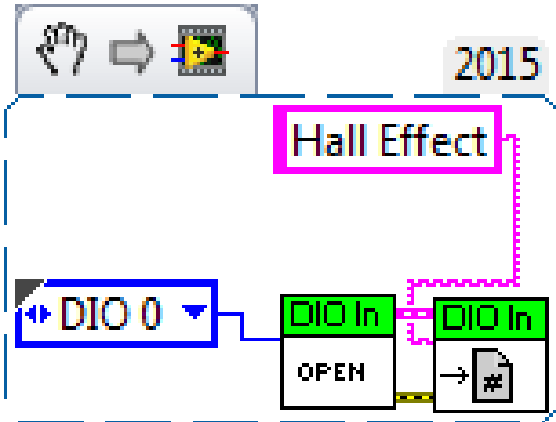
Opening the Hall Effect Sensor
