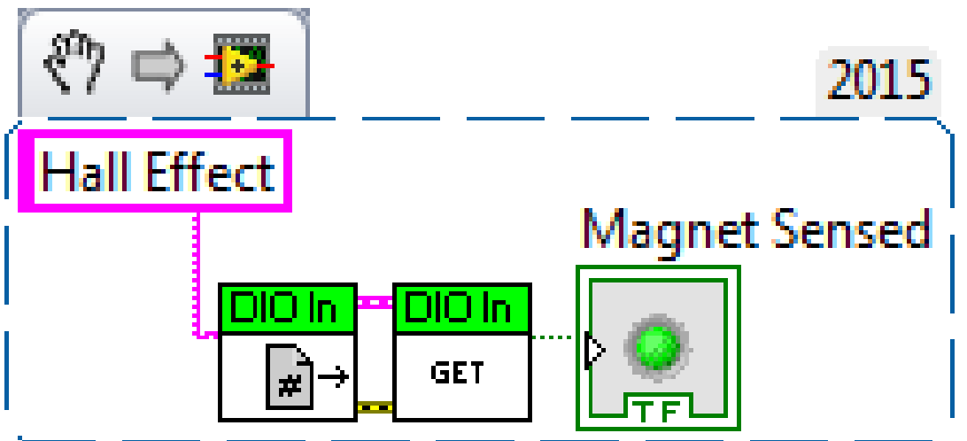
Sensing the Magnet
