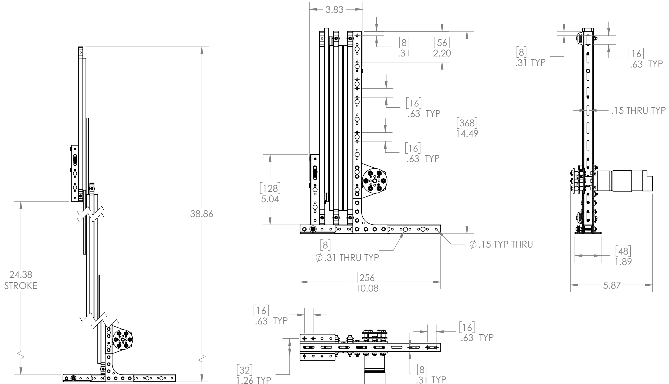
FULLY EXTENDED SCALE 1:5
